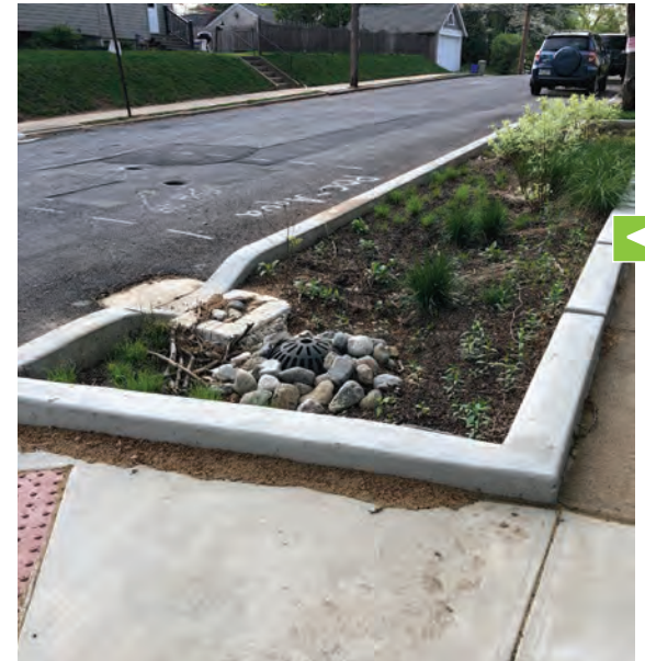
Stormwater planter along residential street in West Chester Borough, PA.
