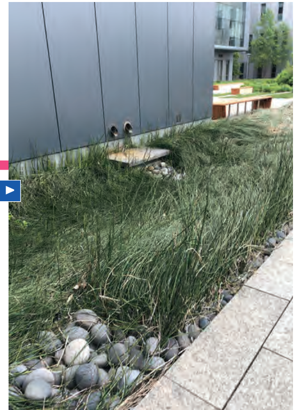
Large downspout planter at University of Delaware, Newark, DE.
