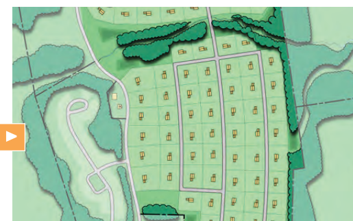
Conventional Layout: Seek to maximize number of lots, but increase length of paved surfaces, utilities and storm water infrastructure
