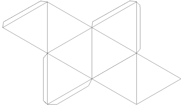
Octahedron
