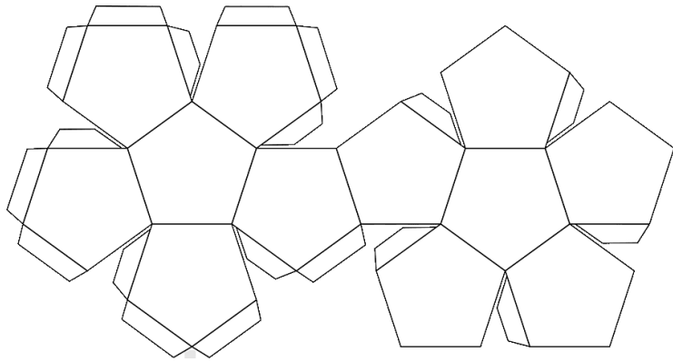
Dodecahedron
