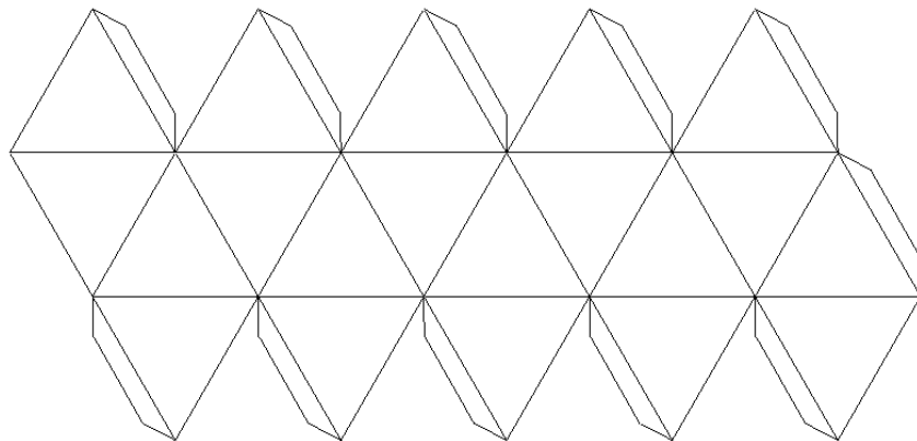
Icosahedron
