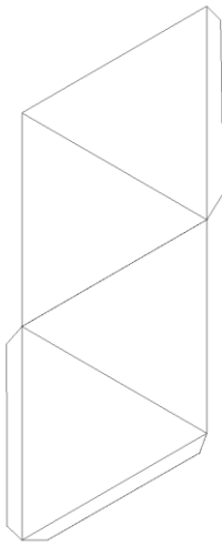
Tetrahedron
